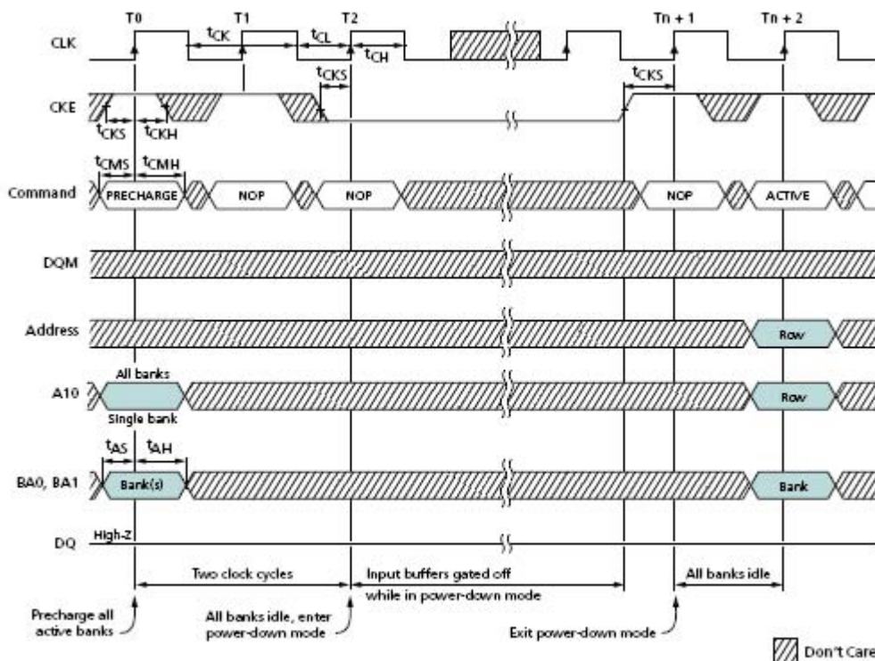
Figure 47: Power-Down Mode
