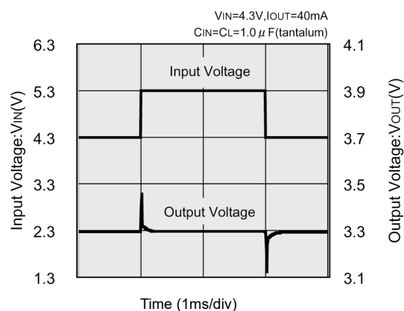
XC6201P332
