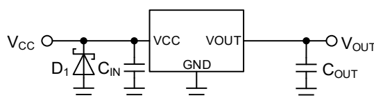
Figure 44. Surges Lower than -0.3 V is Applied to the Input
