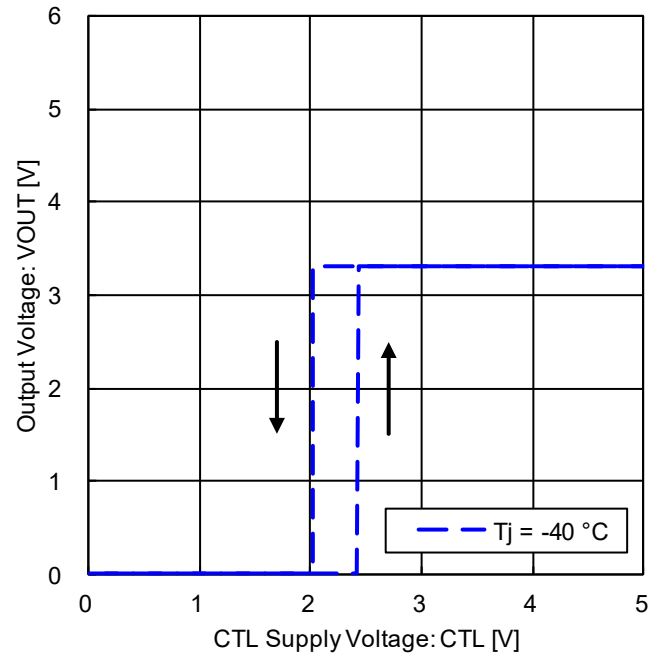
Figure 17. CTL ON / OFF Mode Voltage (Tj = -40 °C)
