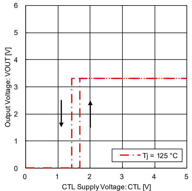
Figure 19. CTL ON / OFF Mode Voltage (Tj = 125 °C)
