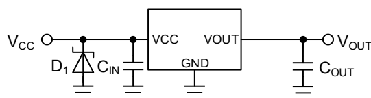
Figure 43. Surges Higher than absolute maximum ratings are Applied to the Input
