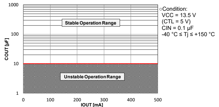
Figure 41. COUT (Typ) vs IOUT
