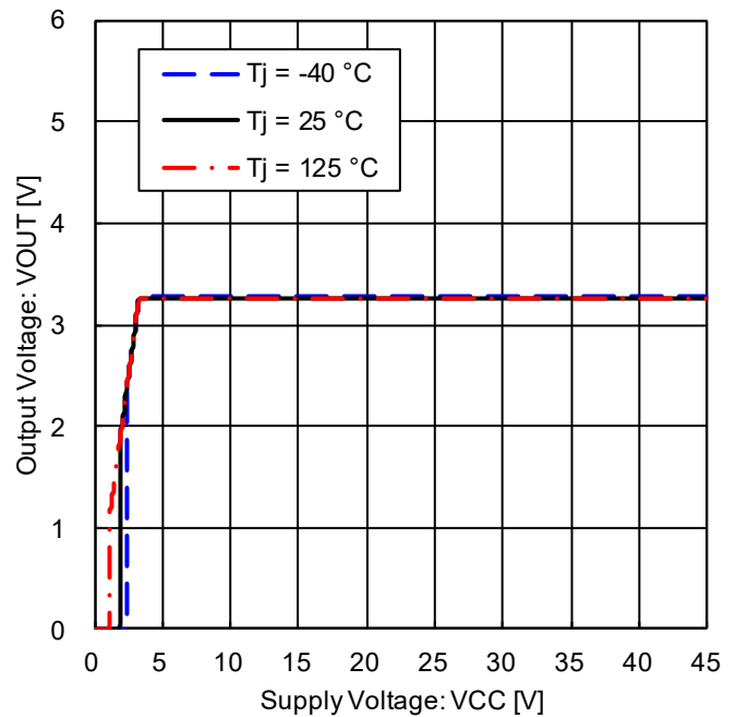
Figure 5. Output Voltage vs Power Supply Voltage ( I_{OUT} = 0\text{ mA} )
