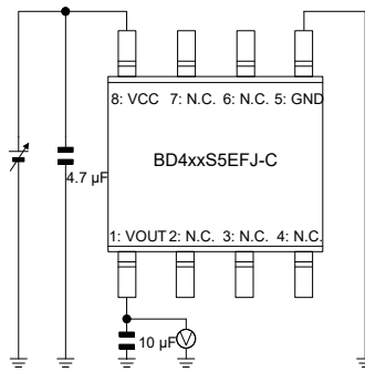
Measurement Setup for Figure 5, 7, 13, 14, Figure 23, 25, 31, 32
