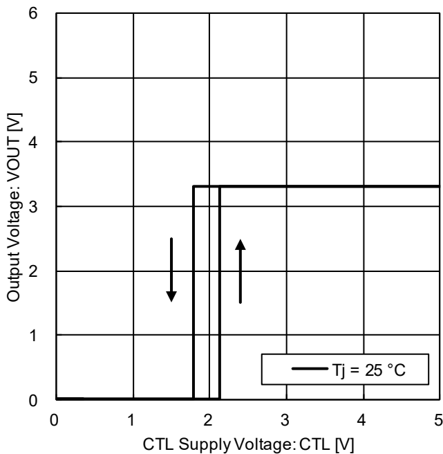
Figure 18. CTL ON / OFF Mode Voltage (Tj = 25 °C)
