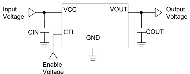
For product with Enable input
