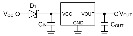
Figure 49. Protection against Reverse Polarity 1
