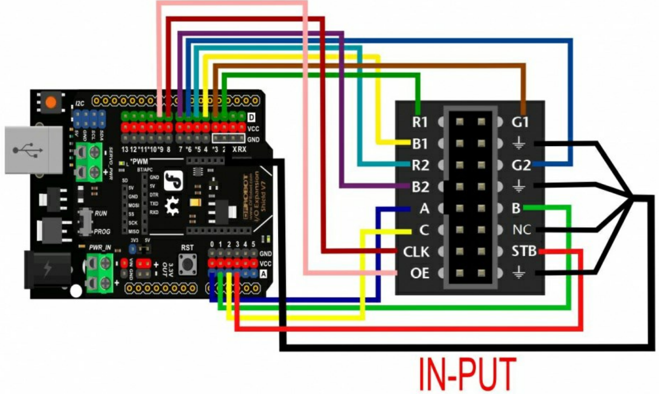
DFR0471 Connection Diagram
