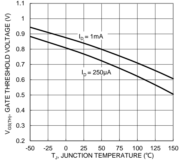
Figure 8. Gate Threshold Voltage vs. Junction Temperature
