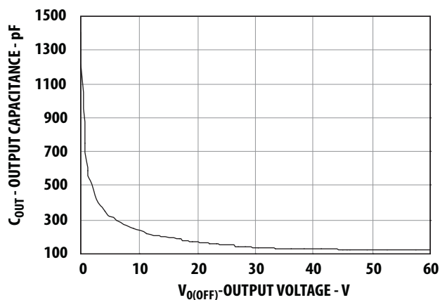
Figure 6: Typical Output Capacitance vs. Output Voltage
