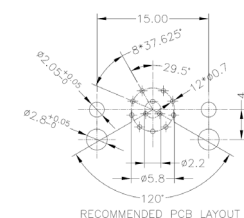
12 Contact PCB Layout
