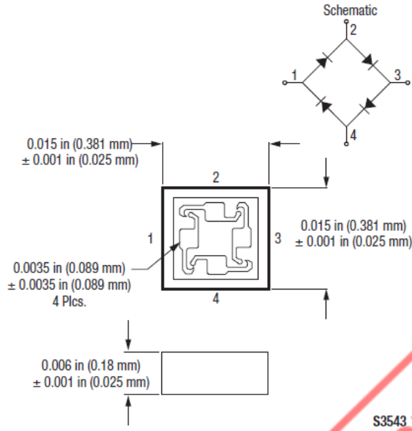
Figure 2. 551-002 Package Dimensions
