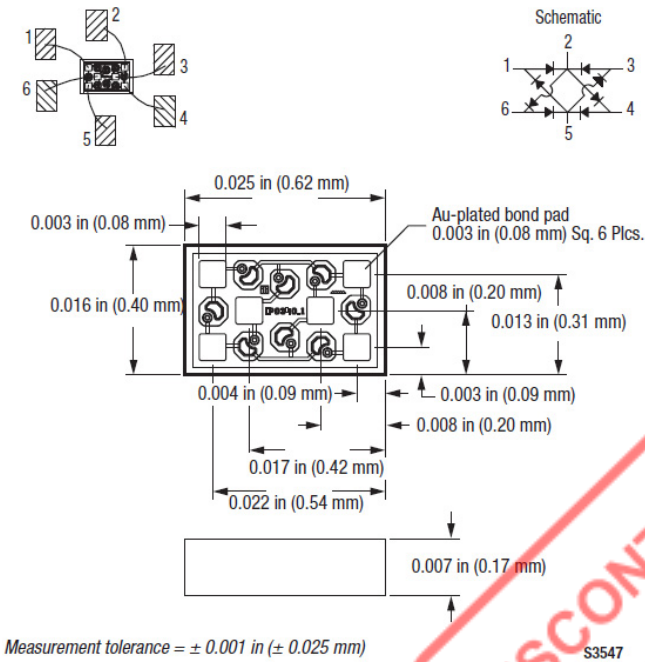
Figure 6. 588-065 Package Dimensions
