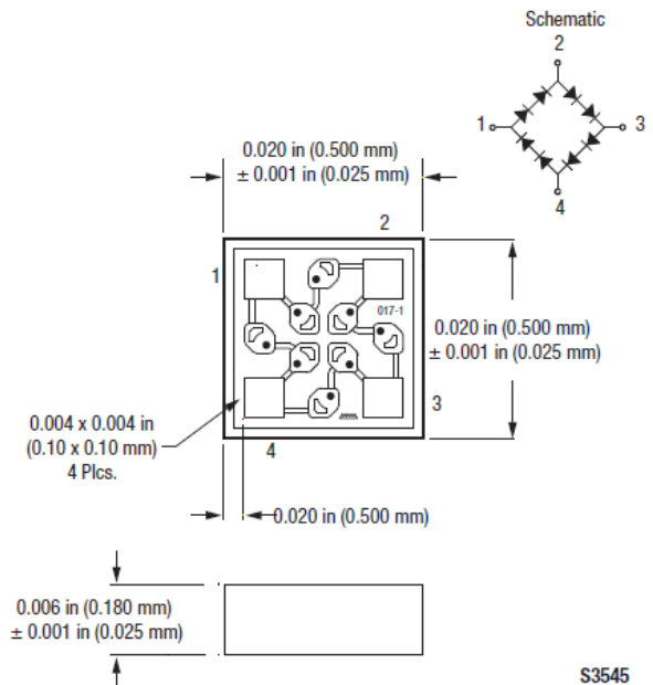
Figure 5. 556-020 Package Dimensions
