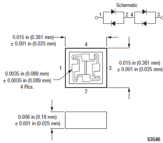
Figure 4. 551-056 Package Dimensions
