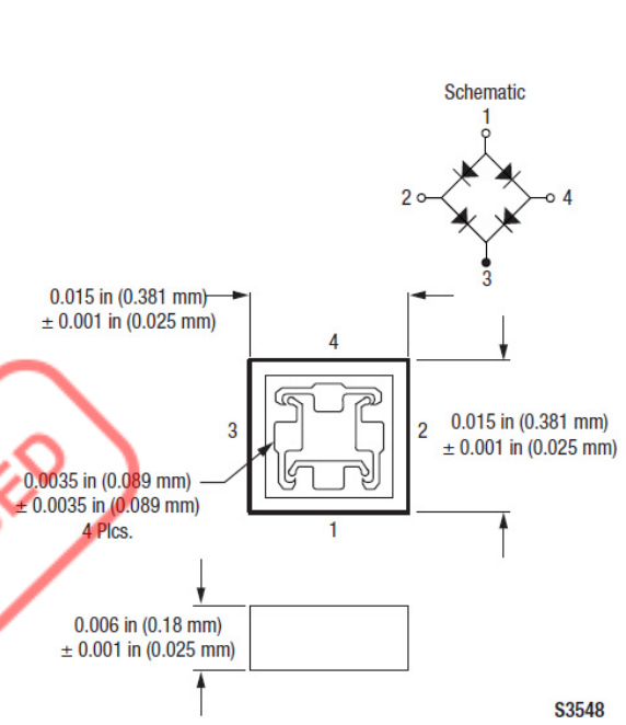
Figure 7. 551-004 Package Dimensions
