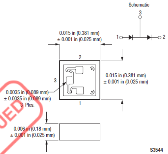
Figure 3. 551-012 Package Dimensions
