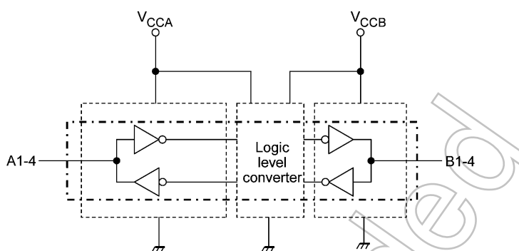
Fig. 6.1 Block Diagram
