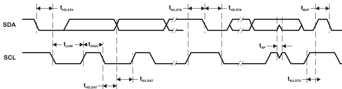
Figure 4-10. I 2 C Mode Timing
