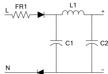
Figure 8: Half-Wave Rectifier
