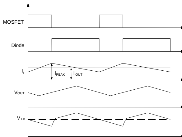
Figure 3: Constant-Voltage Regulation
