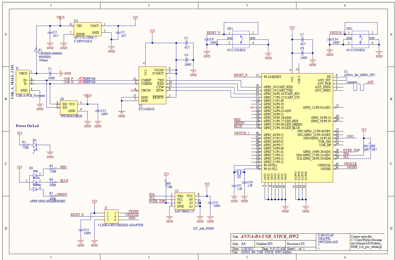
Figure 5: USB-ANNA-B4 schematic
