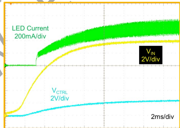
Figure 37 Soft Start with 100nF Capacitor on CTRL Pin
