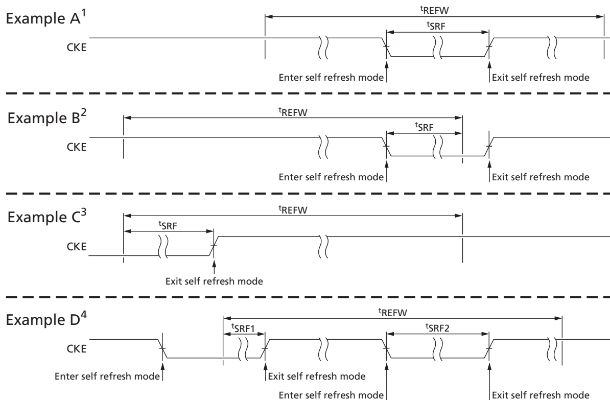
Figure 40: t_{SRF} Definition
