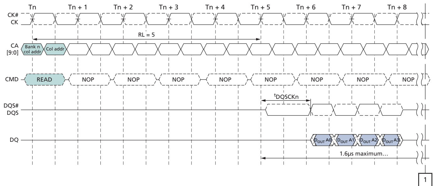
Figure 17: t_{DQSCDM} Timing
