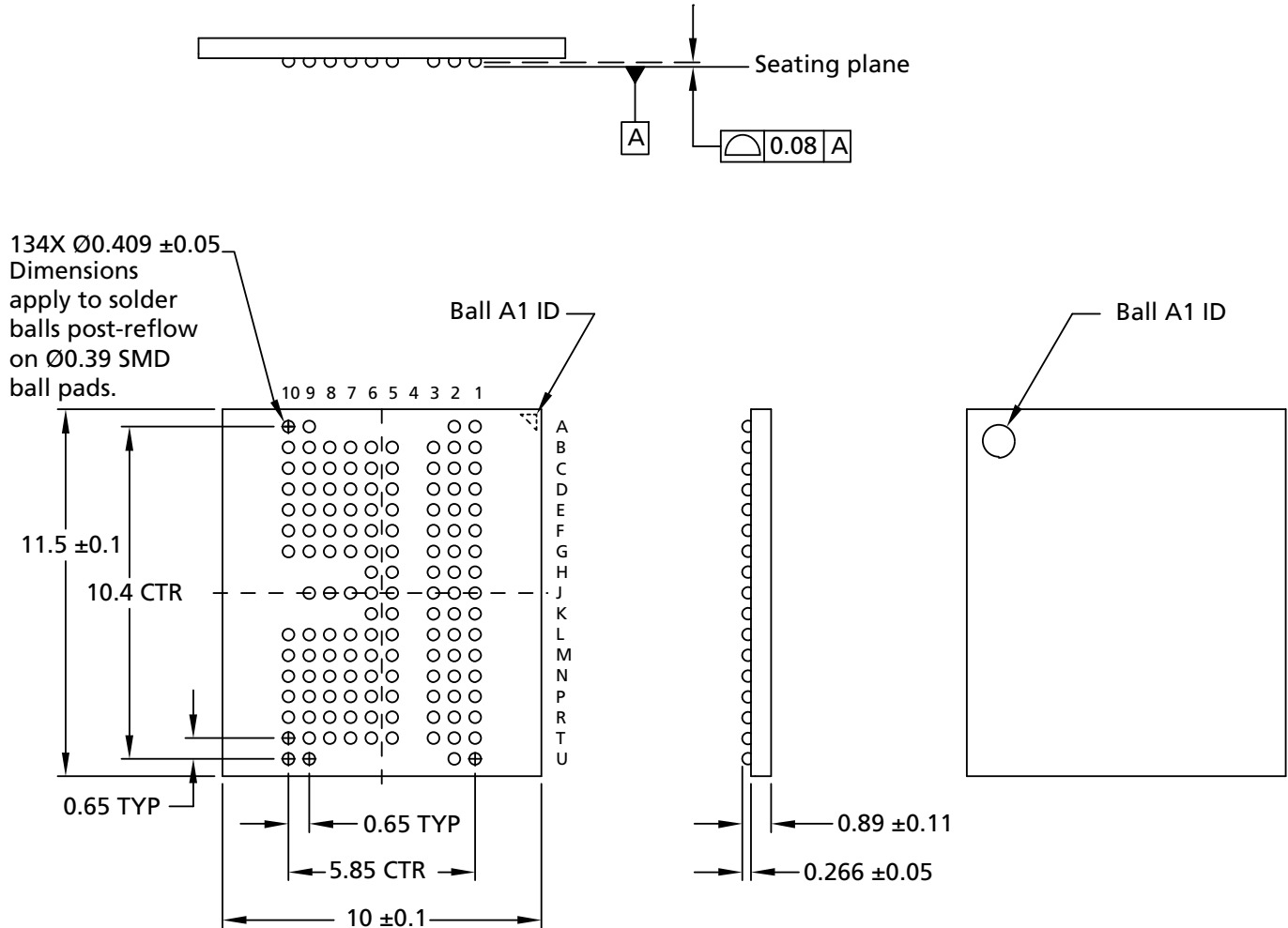
Figure 6: 134-Ball VFBGA – 10mm x 11.5mm (Package Code: HE)
