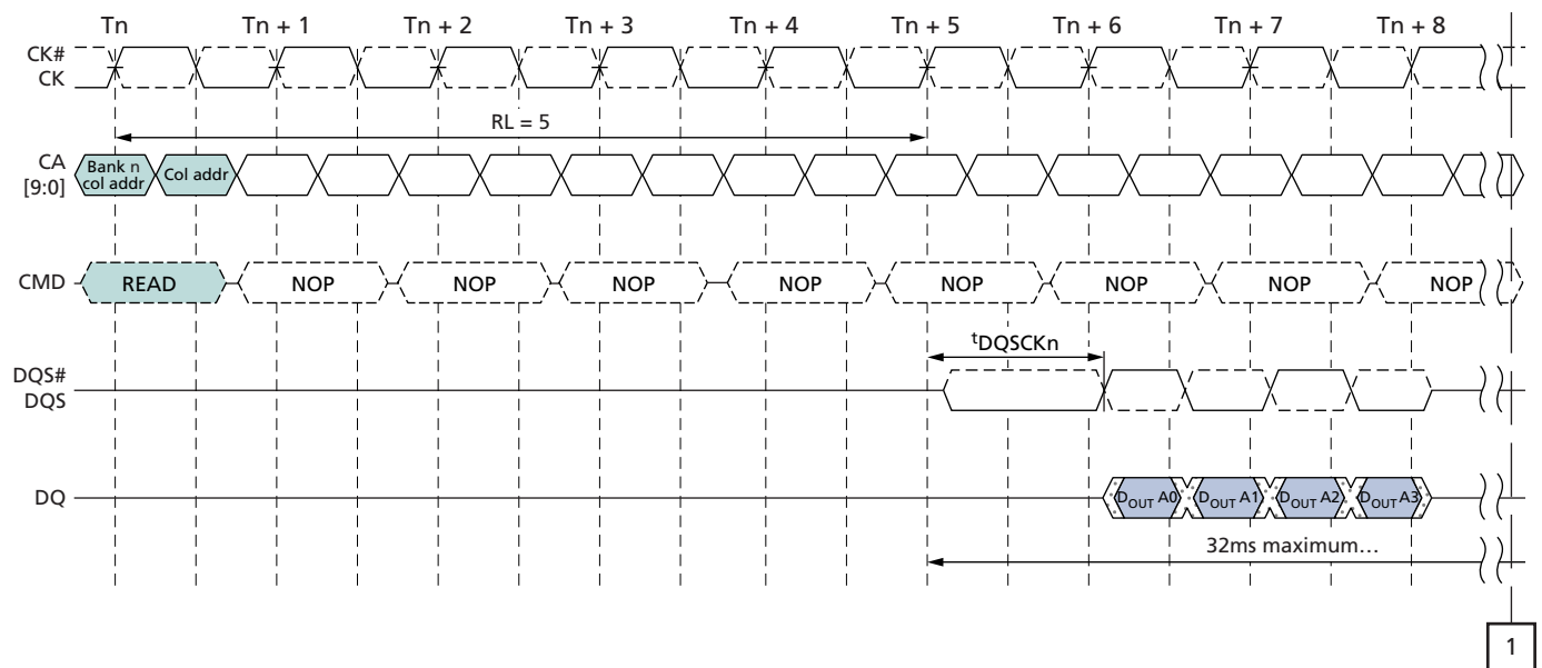
Figure 16: t_{DQSKDL} Timing
