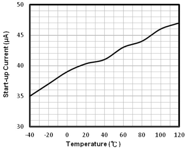
Figure 3 – Start-up Current vs. Ambient Temperature
