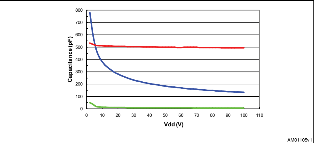
Figure 6. Capacitances vs drain supply voltage
