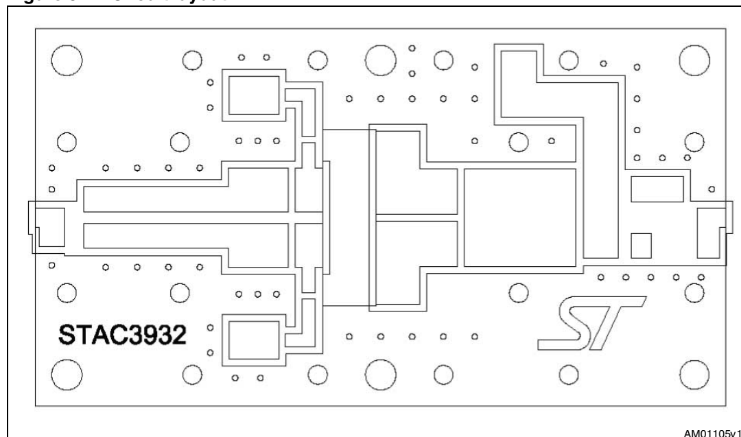
Figure 5. Circuit layout
