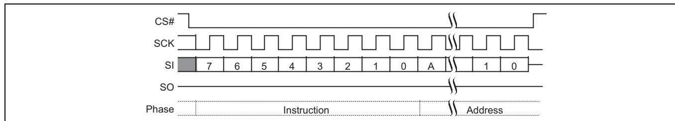
Figure 82 Parameter Sector Erase (P4E 20h or 4P4E 21h) command sequence [63]
