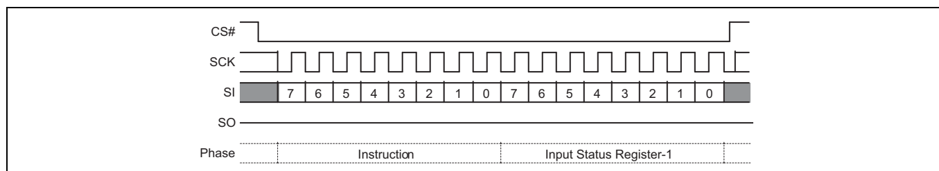
Figure 51 Write Registers (WRR) command sequence – 8 data bits
