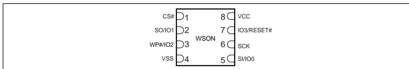
Figure 2 8-connector package (WSO6), top view [9, 10]
