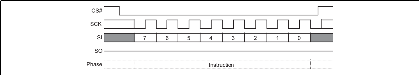
Figure 115 Release from Deep Power-Down command sequence
