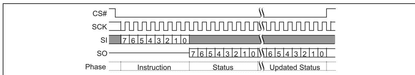
Figure 49 Read Status Register 2 (RDSR2) command
