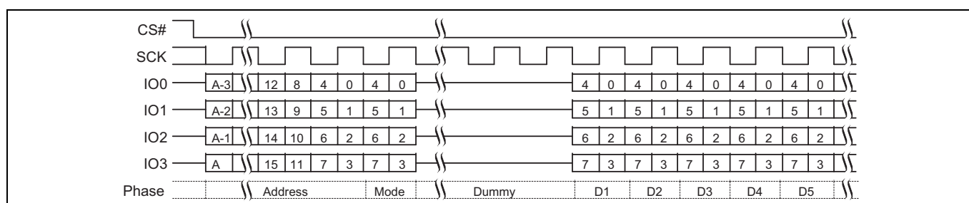
Figure 78 Continuous DDR Quad I/O Read Subsequent Access (EDh or EEh) [60, 61]
