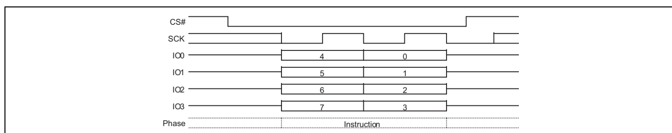
Figure 112 Mode Bit Reset command sequence QPI mode
