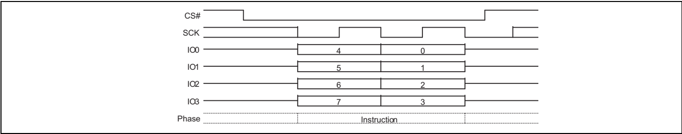
Figure 87 Bulk Erase command sequence QPI mode
