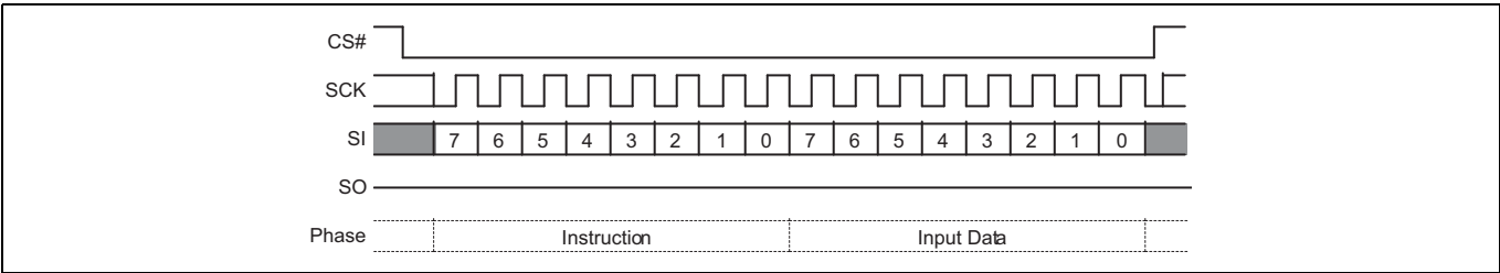
Figure 63 Program NVDLR (PNVDLR) command sequence
