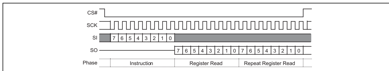
Figure 104 PPB Lock Register Read command sequence
