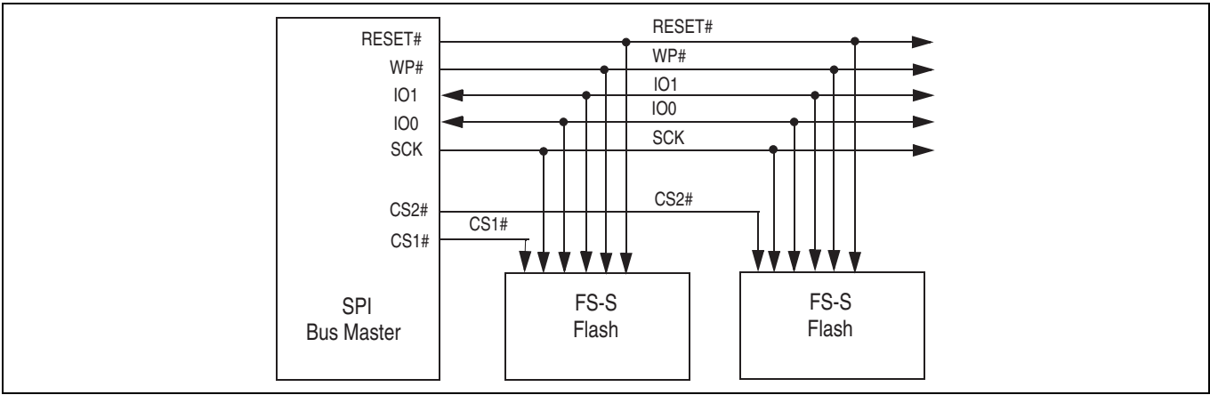
Figure 5 Bus master and memory devices on the SPI bus — dual bit data path
