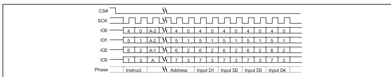
Figure 81 Page Program (PP 02h or 4PP 12h) QPI mode command sequence [62]
