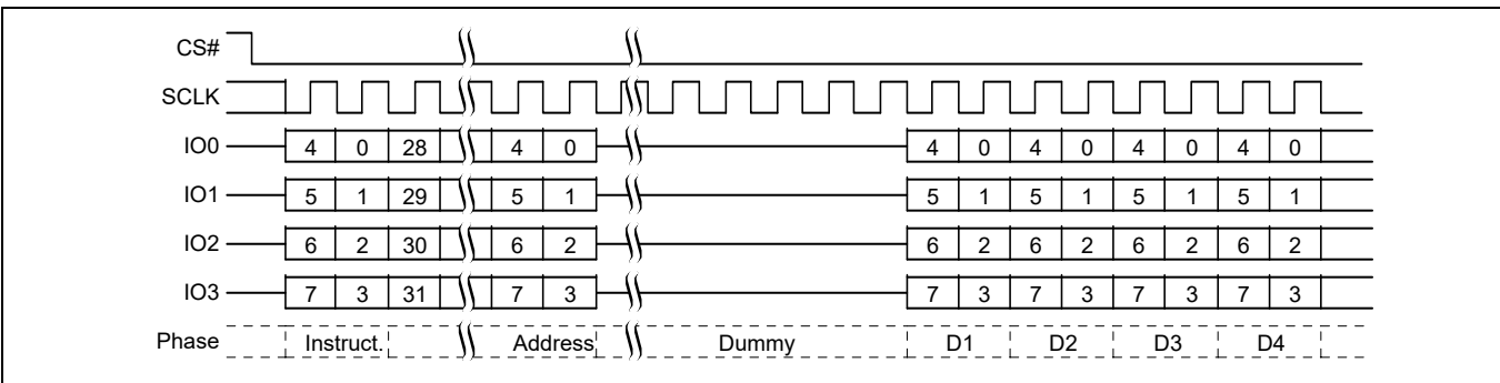
Figure 62 ECCRD (19h), QPI Mode, CR2[7] = 1, or 4EECRD (18h) command sequence
