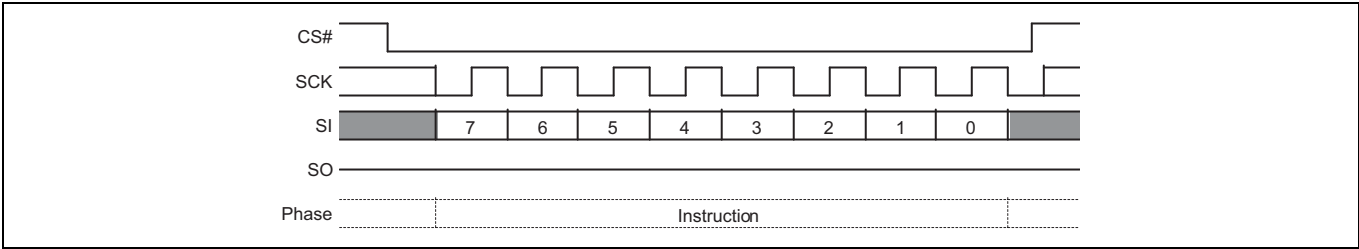
Figure 58 Clear Status Register (CLSR) command sequence
