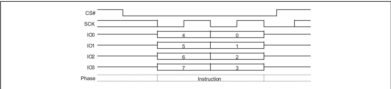
Figure 94 Erase or Program Resume command sequence QPI mode
