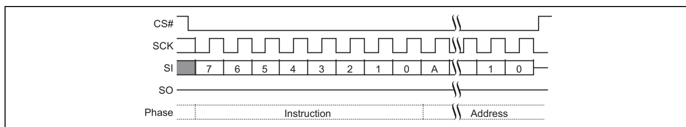
Figure 88 EES command sequence [64]
