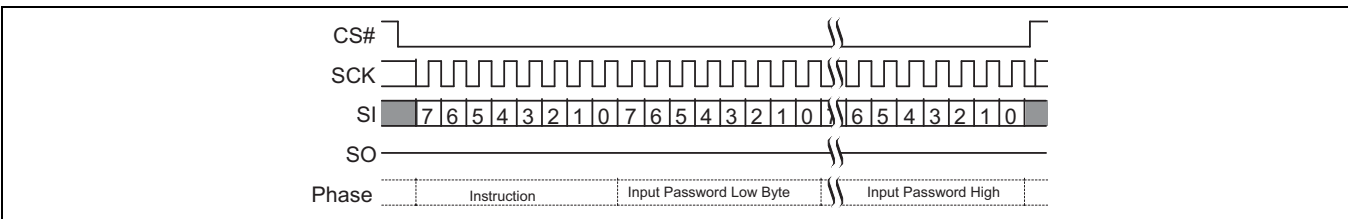
Figure 108 Password Unlock command sequence
