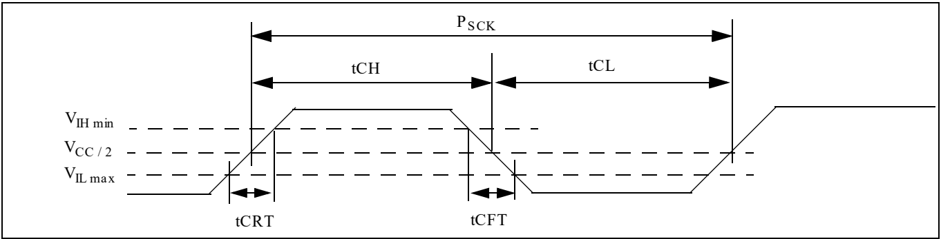
Figure 31 Clock timing
