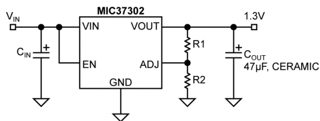
Adjustable Regulator
