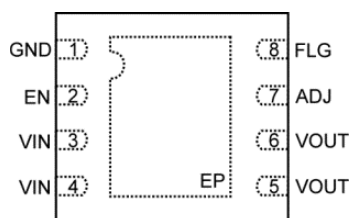
3mm × 3mm DFN (ML) (Top View)
