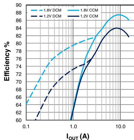
Figure 23: Efficiency, V_{\text{IN}}=19.6\text{V}
