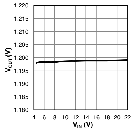
Line Regulation
