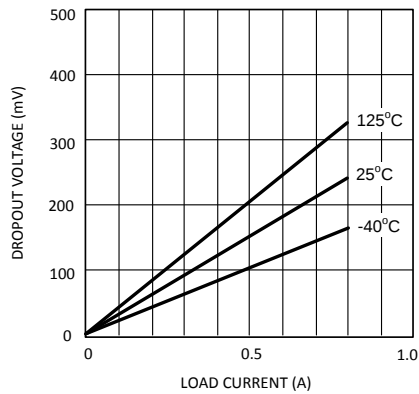
Figure 1. Dropout Voltage vs Output Load Current
