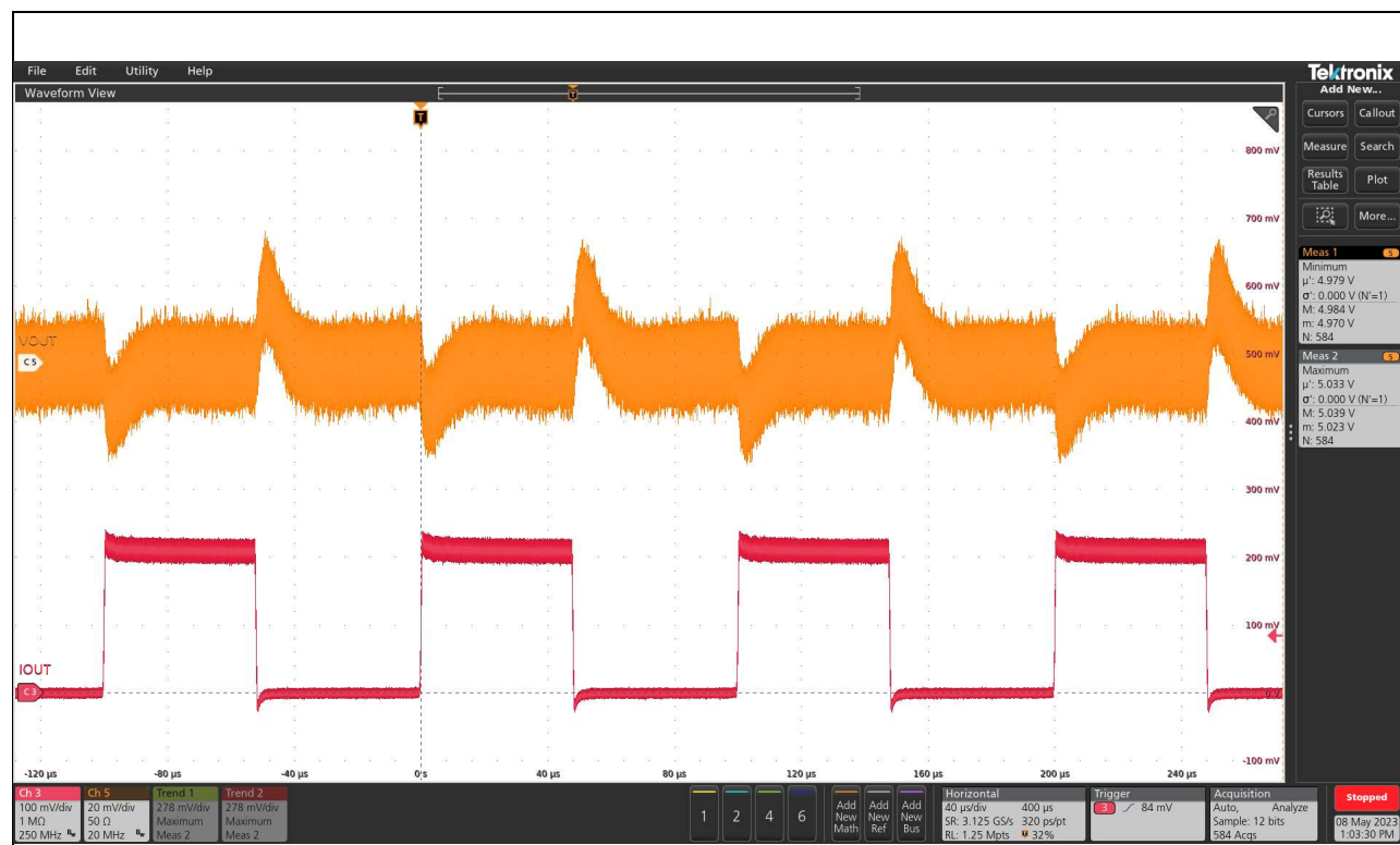
Figure 16 Transient response at 4 A step load current @ 10 A/μs slew rate: I_o = 4\text{ A} - 8\text{ A} , (Ch5: Vo, Ch3: Io), pk-pk: 54mV, fsw = 800 kHz
