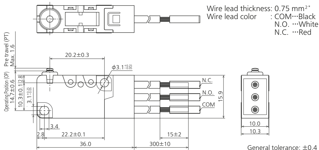
External dimensions
