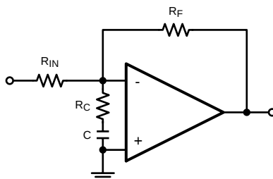
Figure 47. SM73302 with Lead-Lag Compensation for Inverting Configuration
