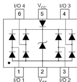
Device Schematic
