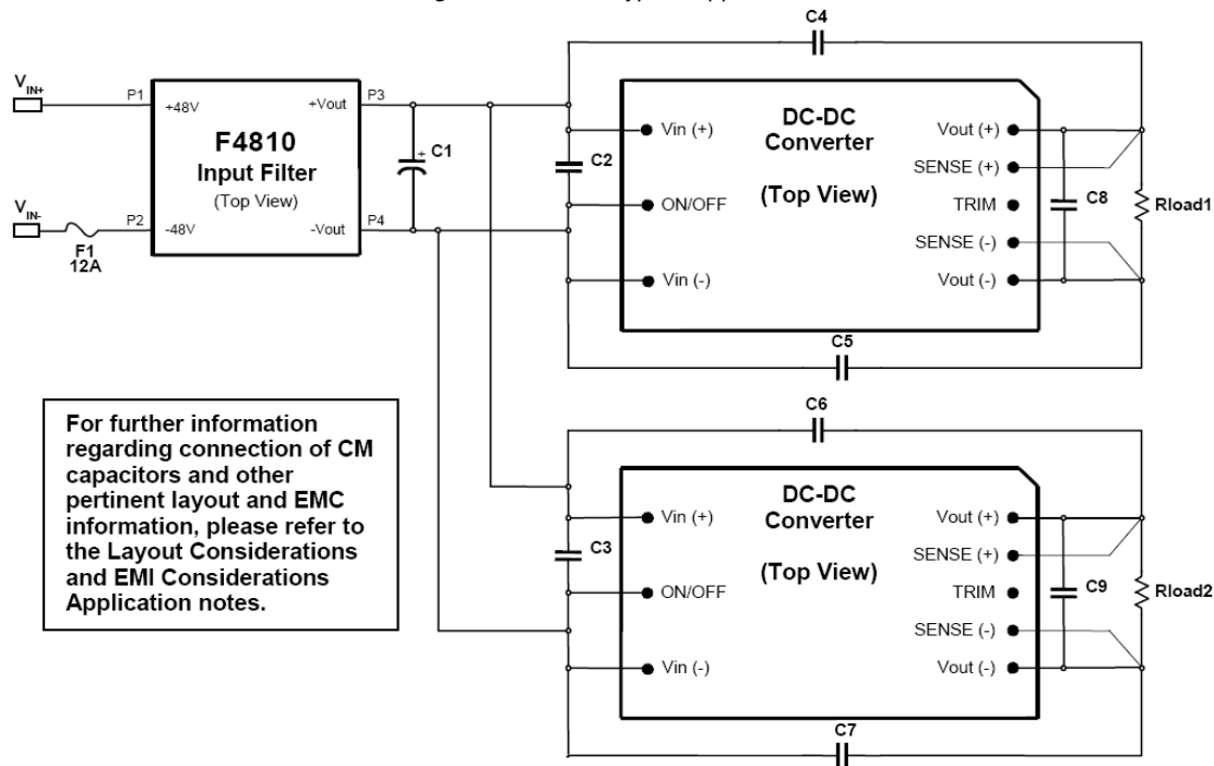
Figure 5 - F4810 – Typical Application
