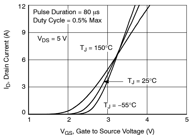
Figure 5. Transfer Characteristics
