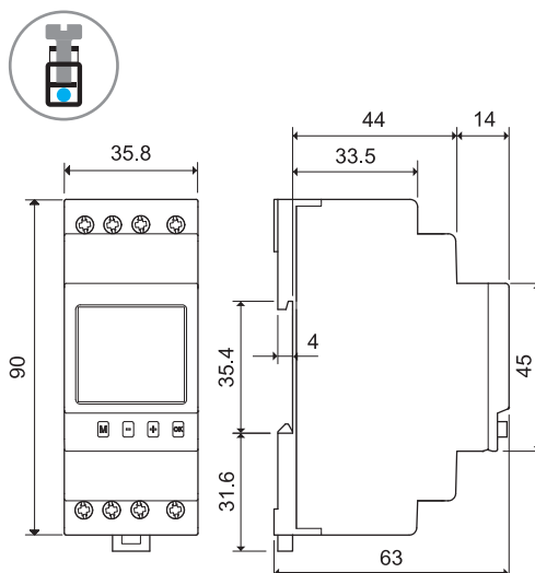
12.51/12.81 Screw terminal
