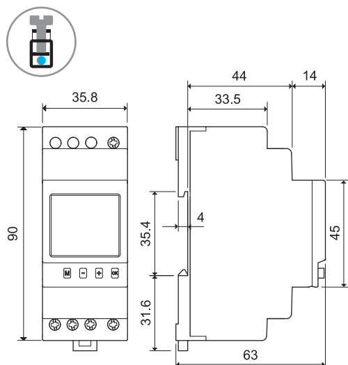
12.31 Screw terminal
