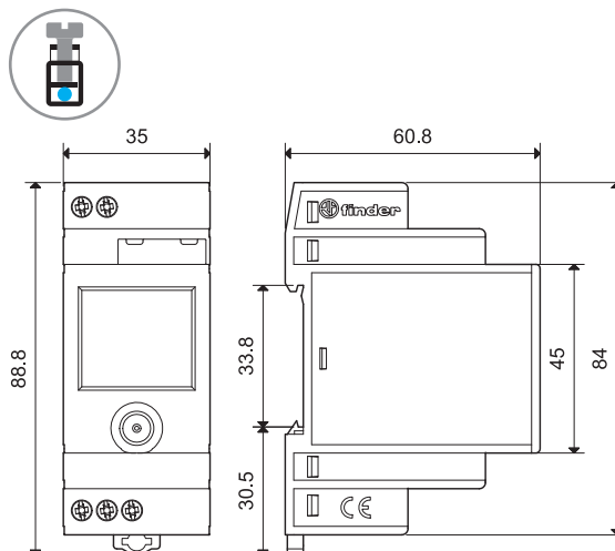
12.51/12.81 Screw terminal
