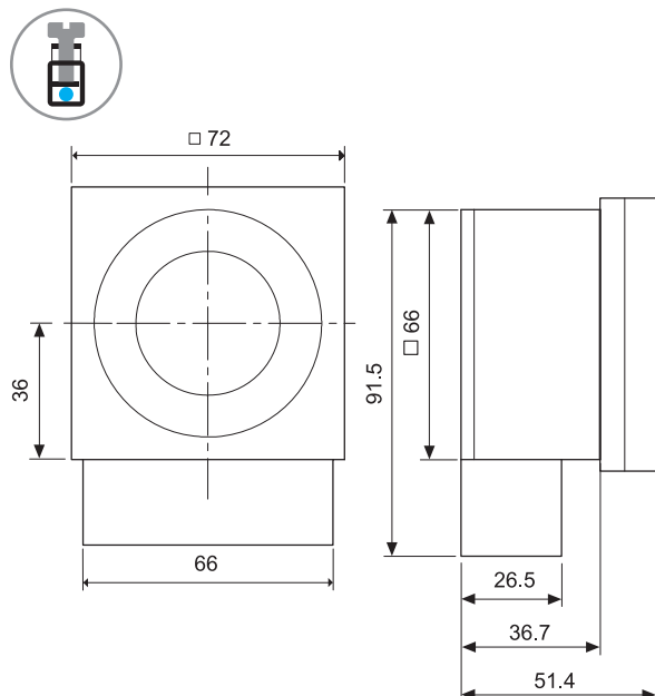
12.31 Screw terminal
