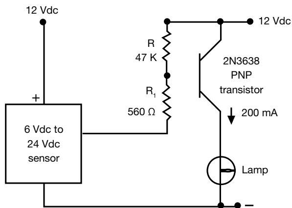
Figure 29. Interface Circuit - dc Load 200 mA
