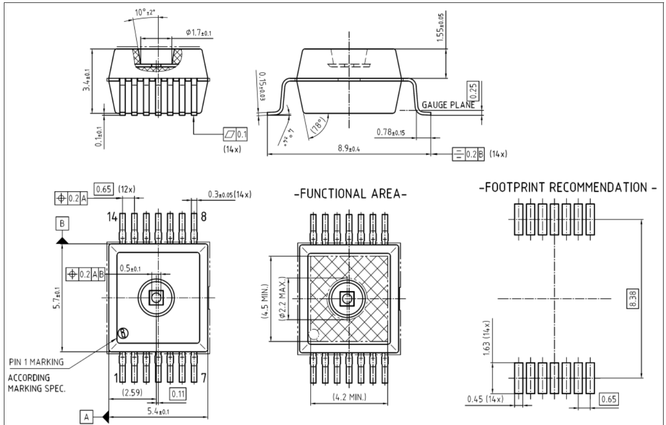
Figure 25 Package Outline
