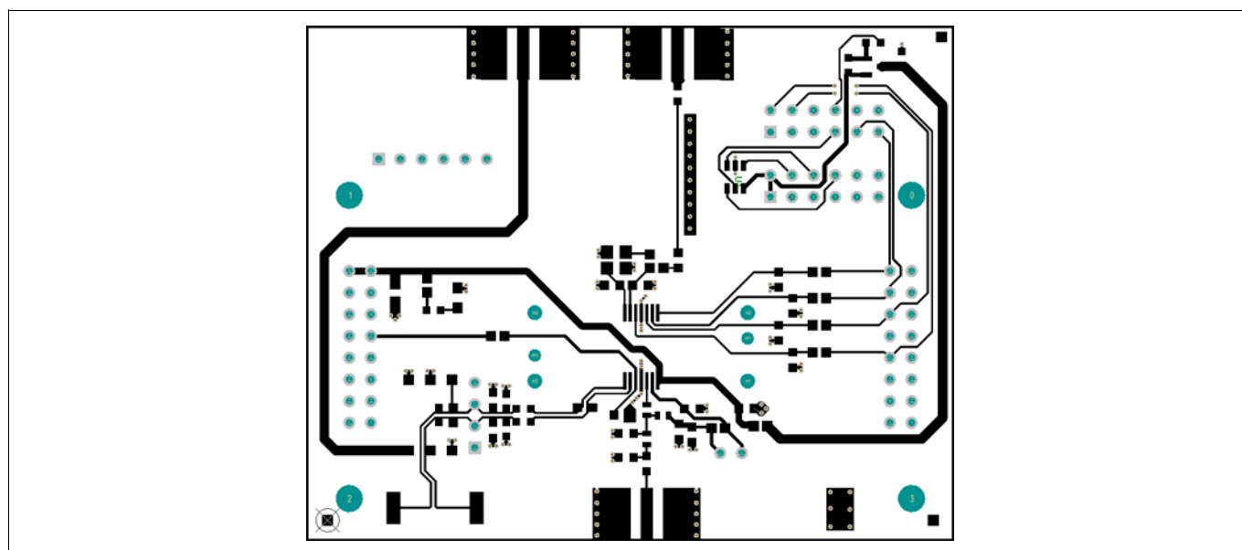
Figure 22 DS Ref Board top layer
