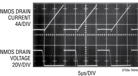
Typical Switching Waveforms
