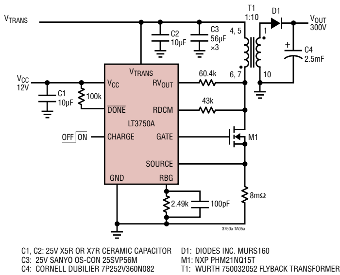
300V, 9A 2.5mF Capacitor Charger
