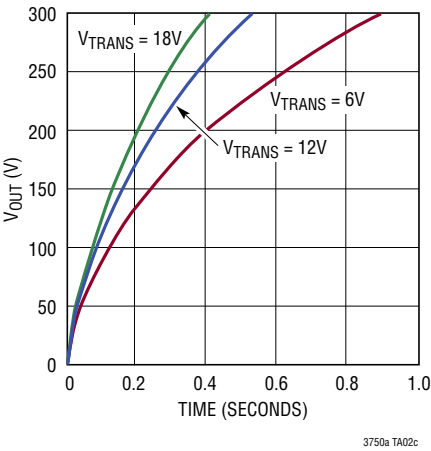
3A Charging Time
