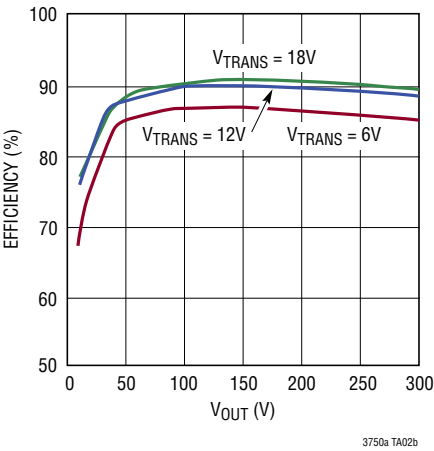
3A Charging Efficiency
