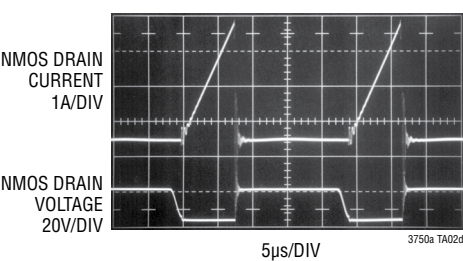
Typical Switching Waveforms
