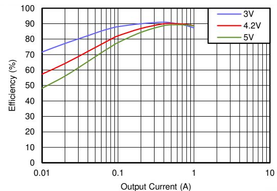
Typical Efficiency for V_{OUT} = 1.8\text{ V} Auto Mode
