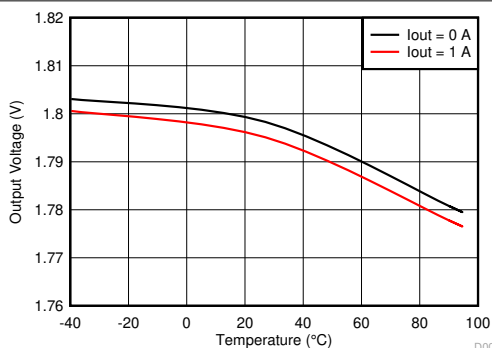
Figure 6-1. Typical Output Voltage vs Temperature
