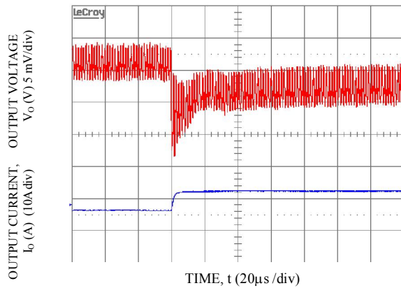
Transient Response to Dynamic Load Change from 50% to 100% at 12Vin, Cout-3x47 \mu F+6x330 \mu F, CTune-47nF, RTune-180ohms. V_o =0.6V
