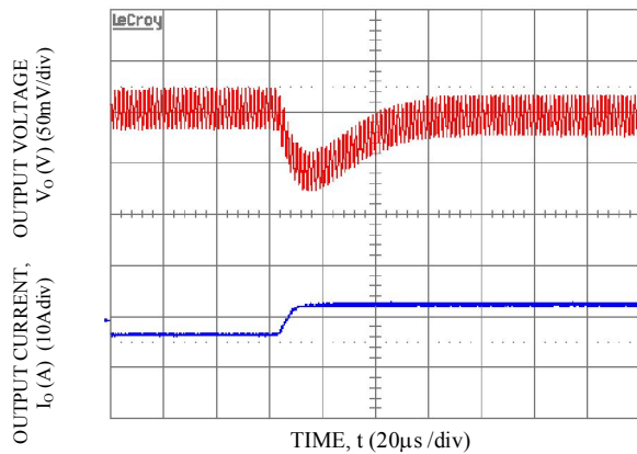
Transient Response to Dynamic Load Change from 50% to 100% at 12Vin, Cout-1x47 \mu F+1x330 \mu F, CTune-2700pF & RTune-330ohms. V_o =3.3V
