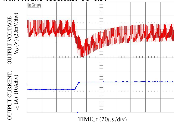
Transient Response to Dynamic Load Change from 50% to 100% at 12Vin, Cout-1x47 \mu F+2x330 \mu F, CTune-5600pF & RTune-270ohms. V_o =1.8V
