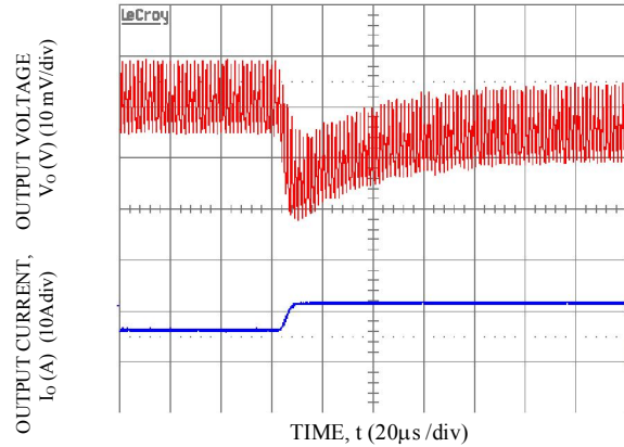
Transient Response to Dynamic Load Change from 50% to 100% at 12Vin, Cout-1x47 \mu F+3x330 \mu F, CTune-10nF & RTune-220ohms. V_o =1.2V
