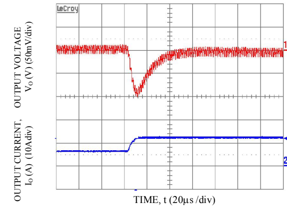
Transient Response to Dynamic Load Change from 50% to 100% at 12Vin, Cout-5x47 \mu F, CTune-1500pF & RTune-330ohms V_o =5.0V
