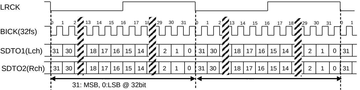
Figure 22. Mode 0/2 Timing (Normal mode, MSB justified, Hex speed mode)
