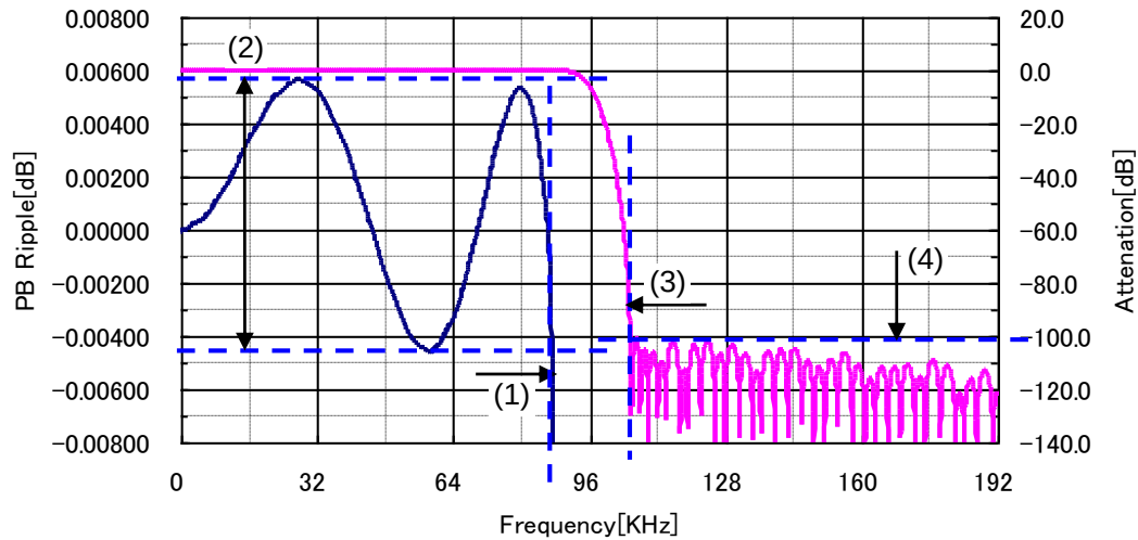
Figure 5. Sharp Roll Off Filter Quad Mode
