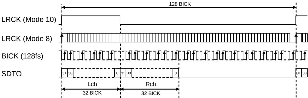
Figure 27. Mode 8/10 Timing (TDM128 mode, MSB justified)
