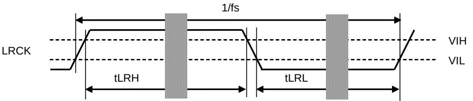
Figure 15. LRCK Timing (TDM0 pin = “L” or “H”)
