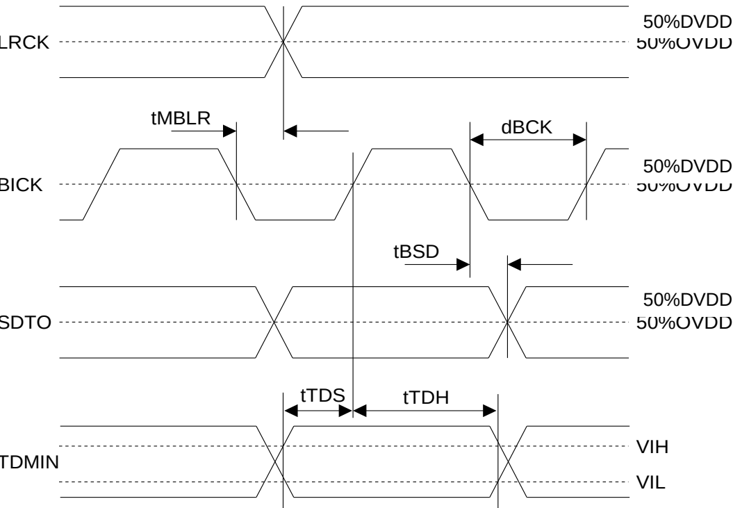
Figure 19. Audio Interface Timing (Master mode, TDM0 pin= “H” or “L”)
