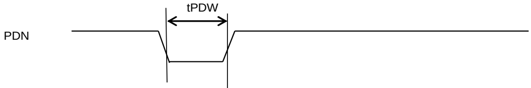
Figure 20. Reset & Calibration Timing
