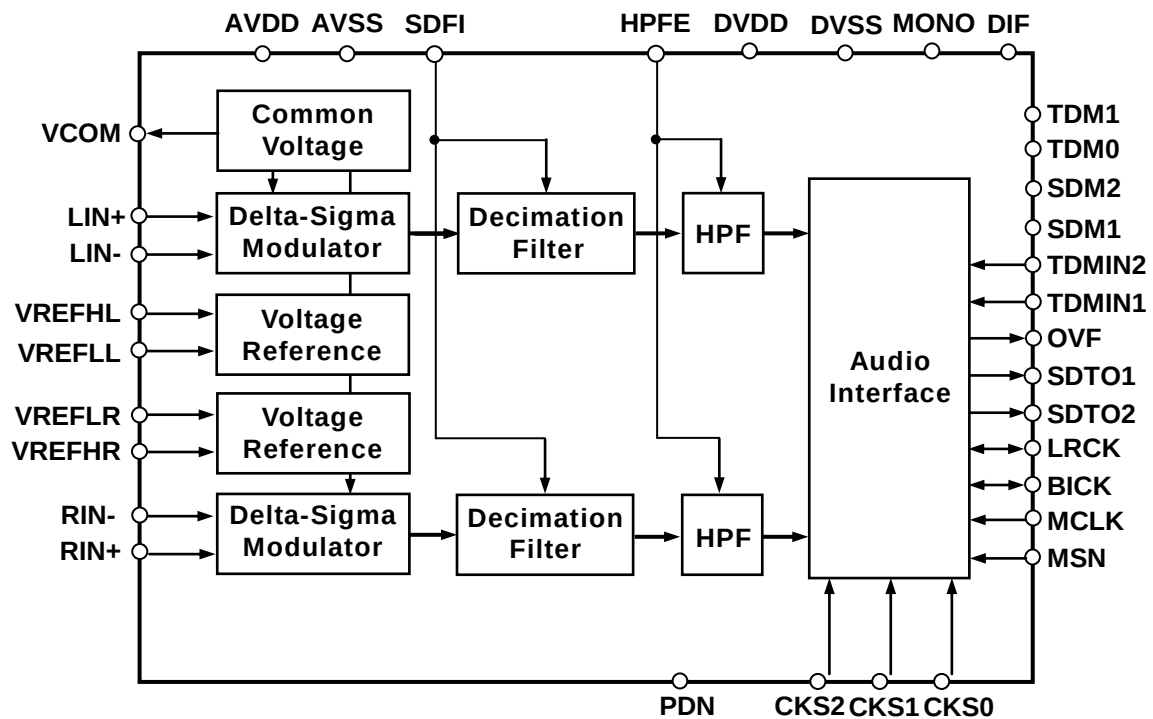
Figure 1. Block Diagram
