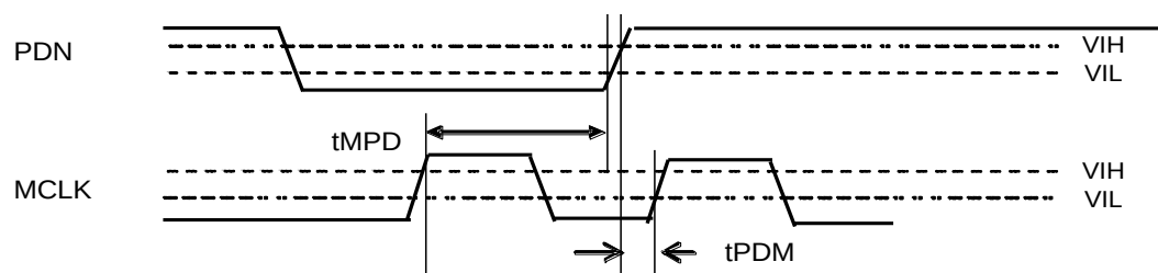
Figure 35. Reset Timing (Slave mode, TDM Mode)
