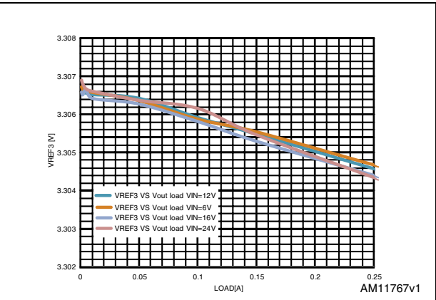
Figure 7. V_{REF3} vs. output load
