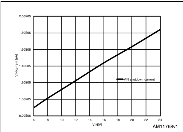
Figure 8. Shutdown V_{IN} current vs. V_{IN} ( EN=0V )
