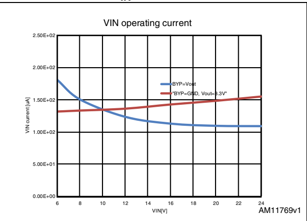
Figure 9. No load V_{IN} current vs. V_{IN} ( EN=V_{IN} )
