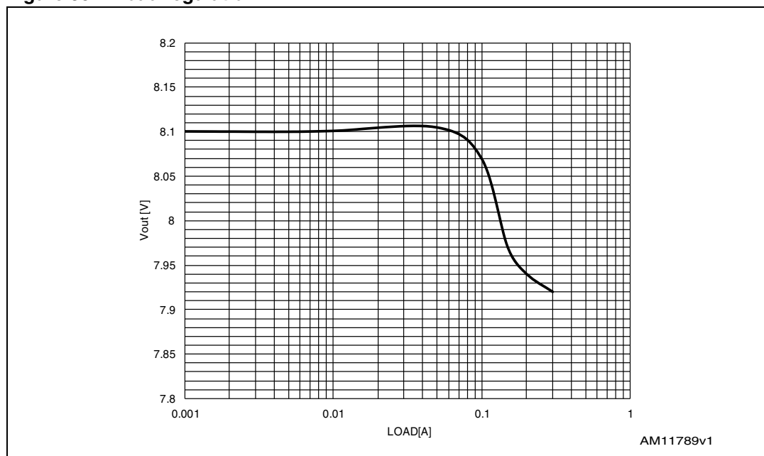
Figure 30. Load regulation
