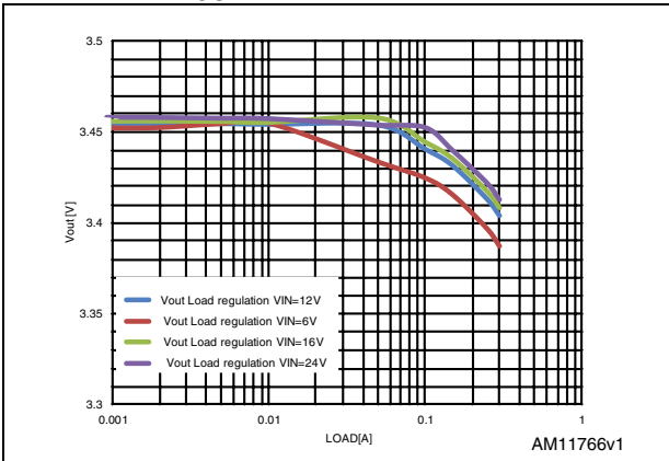
Figure 6. V_{OUT} vs. load
