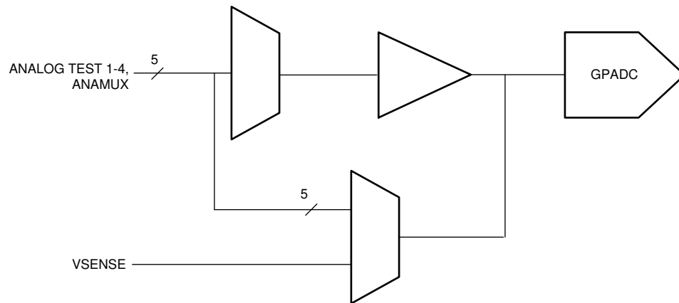
Figure 6-6. ADC Path
