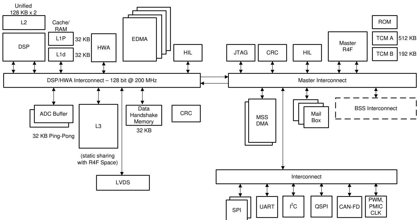
Figure 6-5. Processor Subsystem
