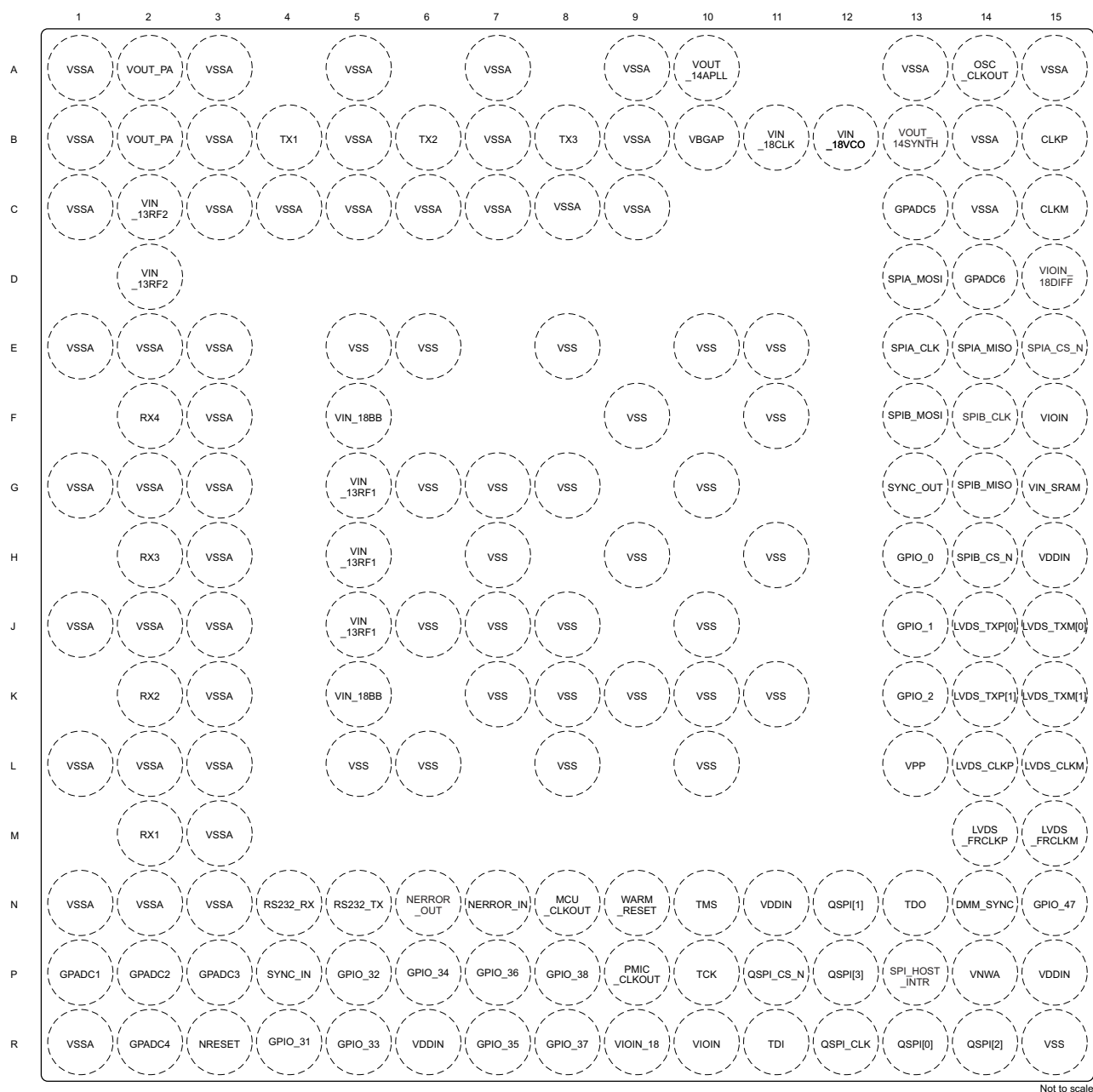
Figure 4-1. Pin Diagram
