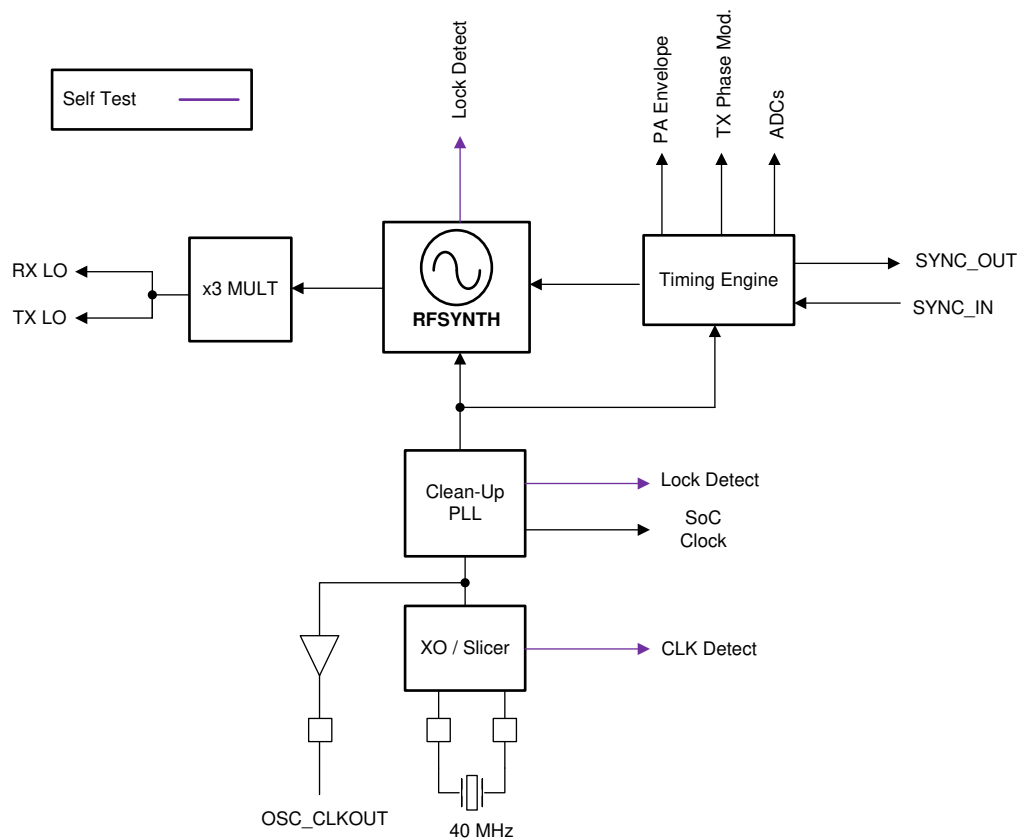
Figure 6-2. Clock Subsystem
