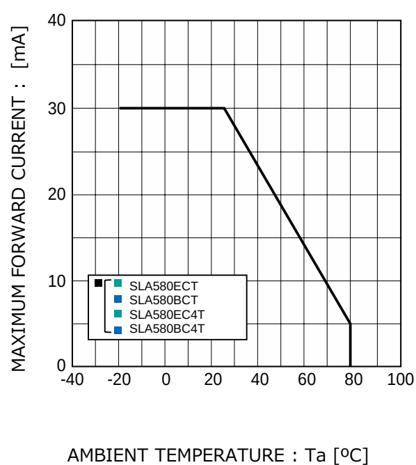
Fig.4 Derating
