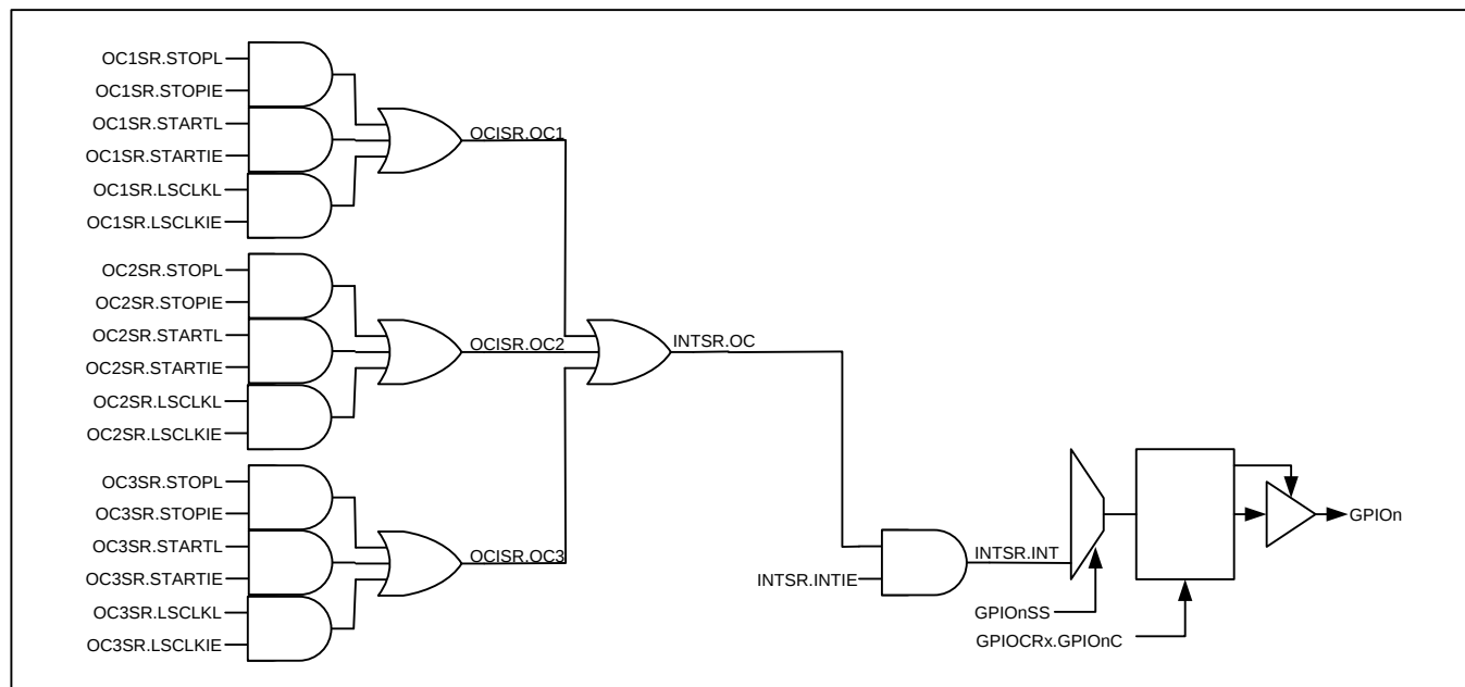
Figure 11 – Interrupt Structure
