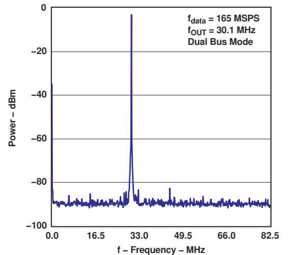
Figure 6-8. Single-Tone Spectrum
