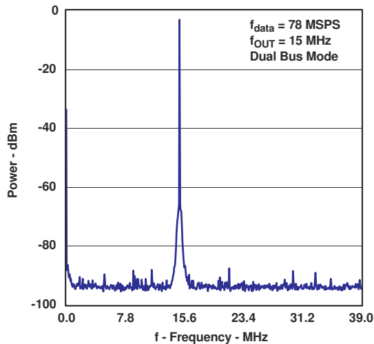
Figure 6-7. Single-Tone Spectrum
