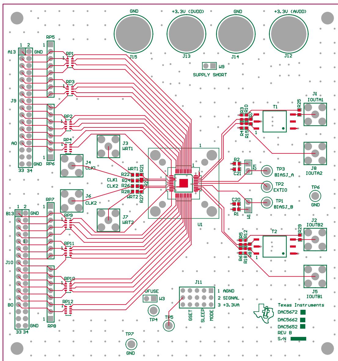
Figure 11-1. Top Layer 1
