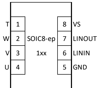
Figure 6 – Pin-out diagram SO8-ep, -1xx variant (Stepper motor, AutoAddress)
