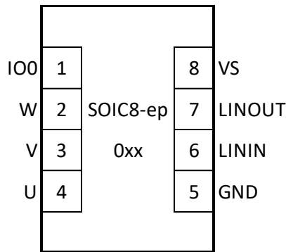
Figure 5 – Pin-out diagram SO8-ep, -0xx variant (BLDC motor, AutoAddress)
