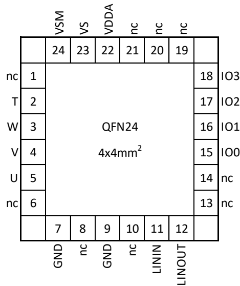
Figure 4 – Pin-out diagram QFN24
