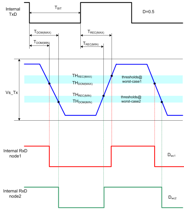
Figure 15 – LIN timing diagram, relation between propagation delay and duty cycle (reference SAE J2602 specification)
