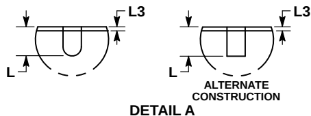
QFNW24 5x5, 0.65P CASE 484AF ISSUE A
