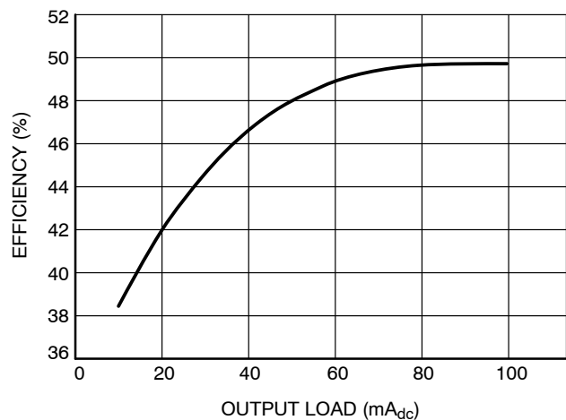
Figure 24. Efficiency vs. Output Current for the Voltage Inverting Demo Board at V_{in} = +5\text{ V} , V_{out} = -12\text{ V} , T_A = 25^\circ\text{C}
