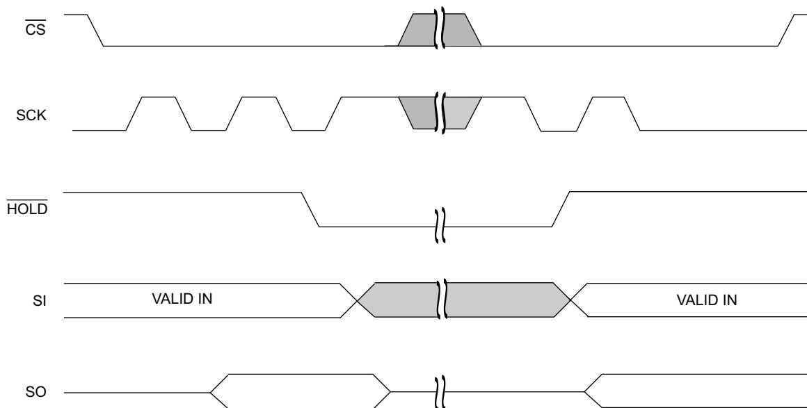
Figure 14. \overline{\text{HOLD}} Operation [2]
