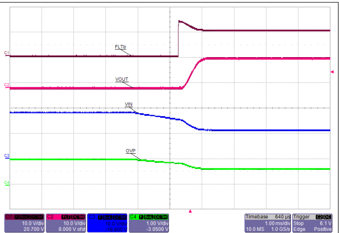
Figure 61. Overtoltage Recovery
