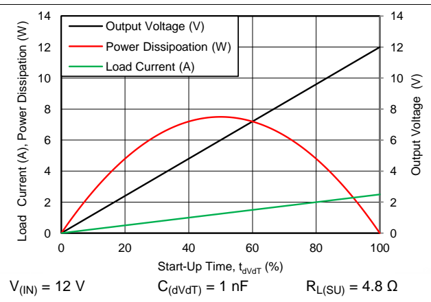
Figure 56. P_{D(LOAD)} in Load During Start-up
