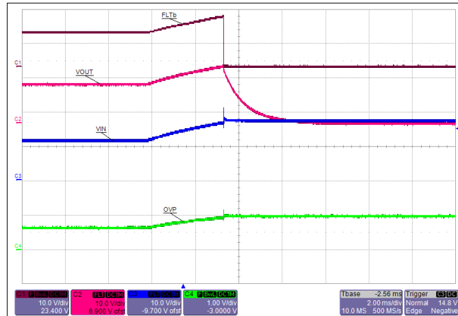
Figure 60. Overtoltage Shutdown
