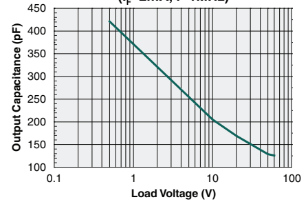
Form-B Output Capacitance vs. Load Voltage ( I_F=2\text{mA} , f=1\text{MHz} )
