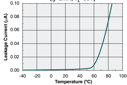
Form-B Typical Leakage vs. Temperature Measured Across Pins 7&8 ( I_F=2\text{mA} , V_L=60\text{V} )
