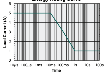
Form-B Energy Rating Curve
