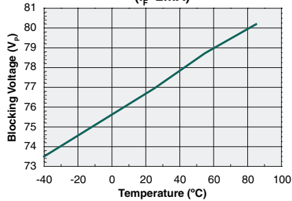
Form-B Typical Blocking Voltage vs. Temperature ( I_F=2\text{mA} )
