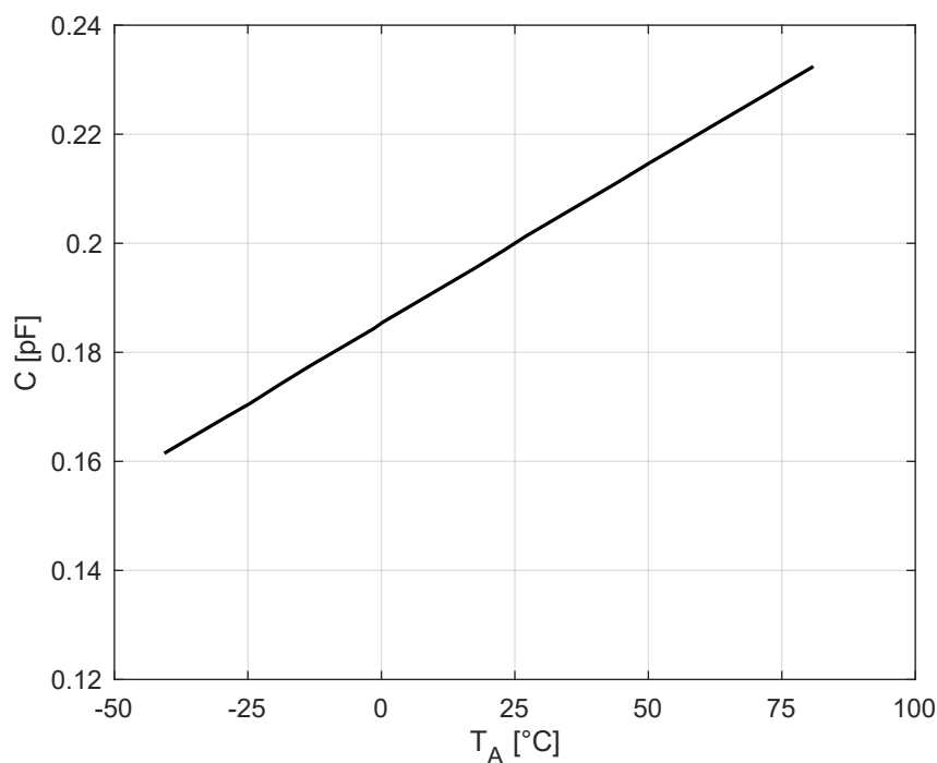
Figure 2 Capacitance C vs. ambient temperature T_A at frequency f = 1 MHz and reverse voltage V_R = 0 V
