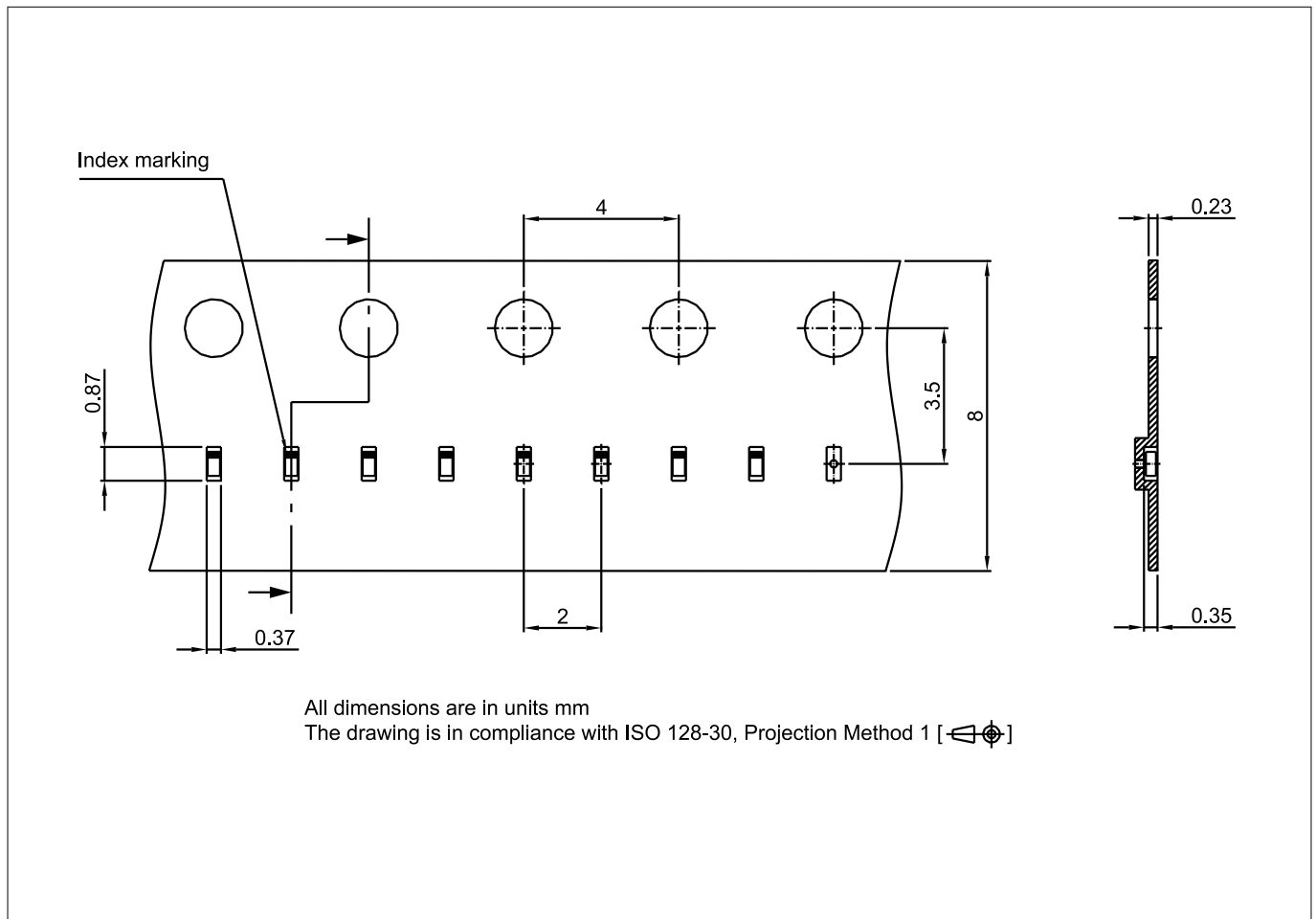
Figure 14 Tape information
