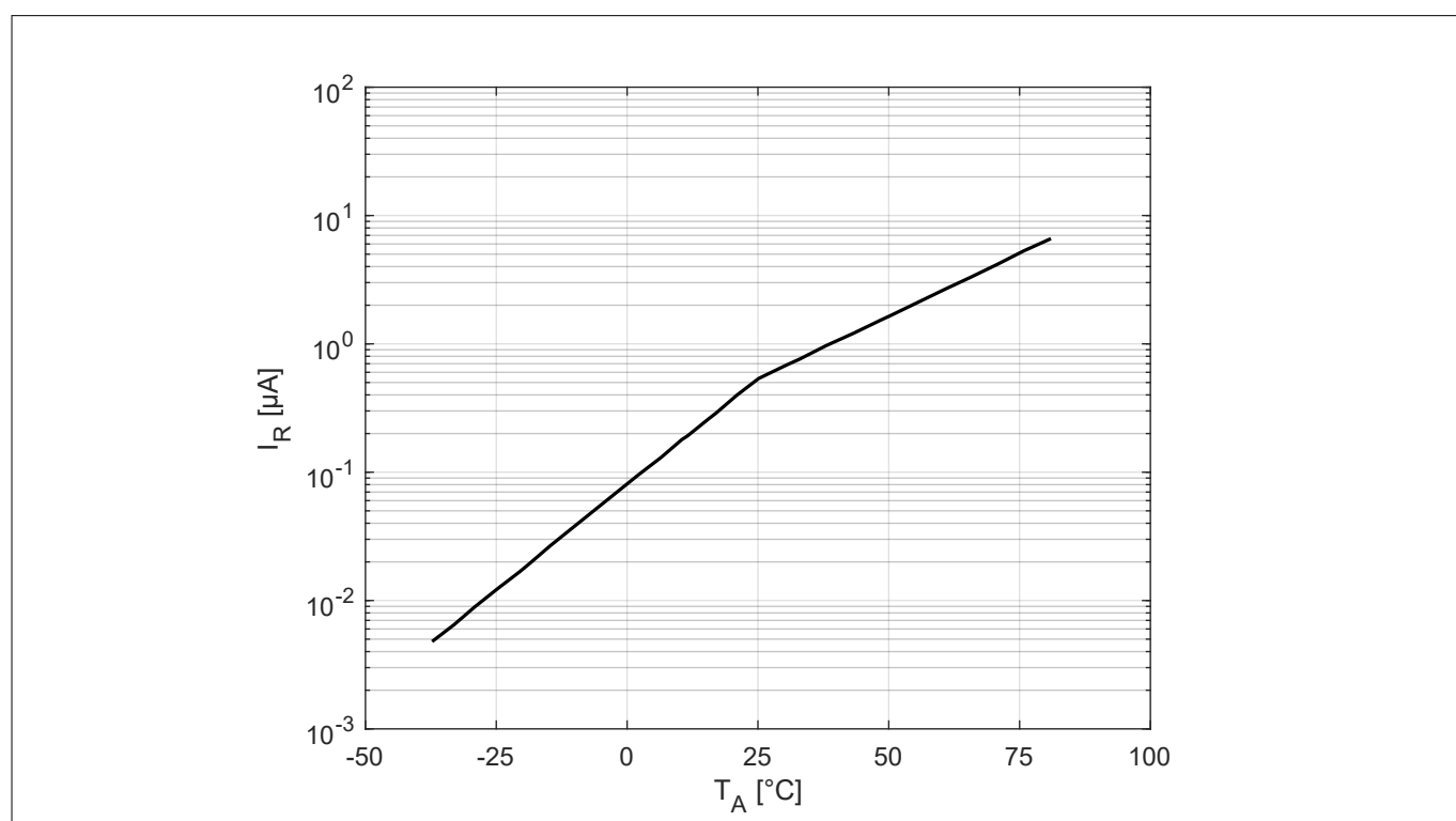
Figure 7 Reverse current I_R vs. ambient temperature T_A at reverse voltage V_R = 1 V
