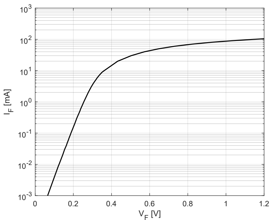
Figure 3 Forward current I_F vs. forward voltage V_F
