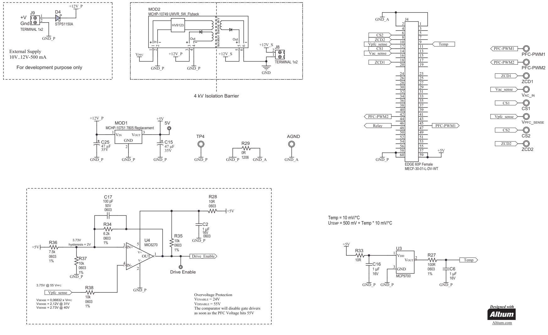
FIGURE A-2: LOW-VOLTAGE POWER FACTOR CORRECTION DEVELOPMENT BOARD SCHEMATICS (PAGE 2 OF 2)
