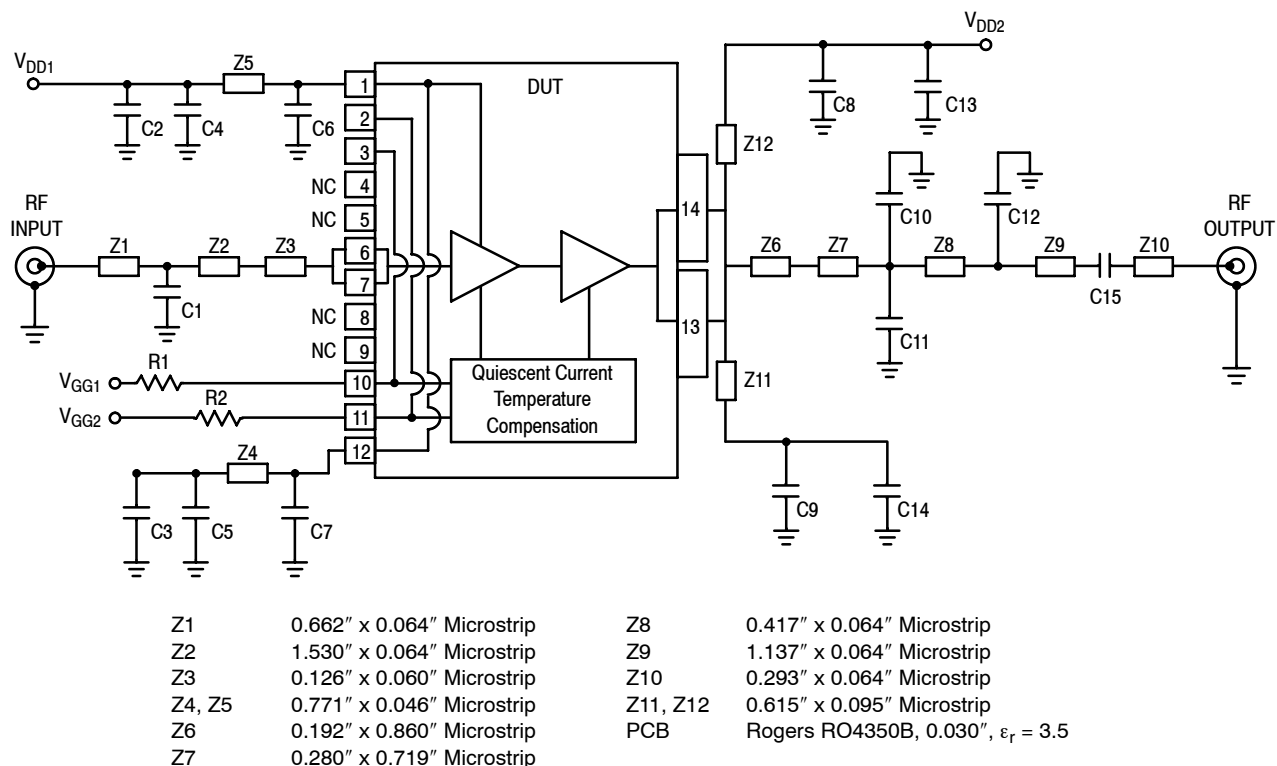
Figure 3. MW7IC2750NR1(GNR1)(NBR1) Test Circuit Schematic
