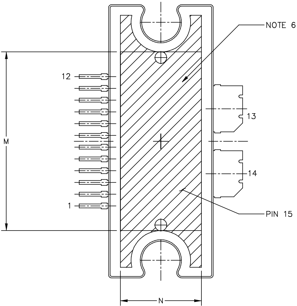
VIEW Y-Y
