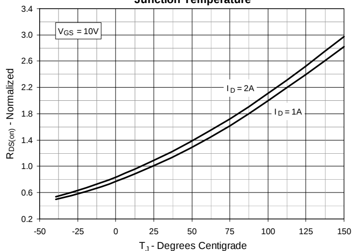
Fig. 3. R_{DS(on)} Normalized to I_D = 1A Value vs. Junction Temperature
