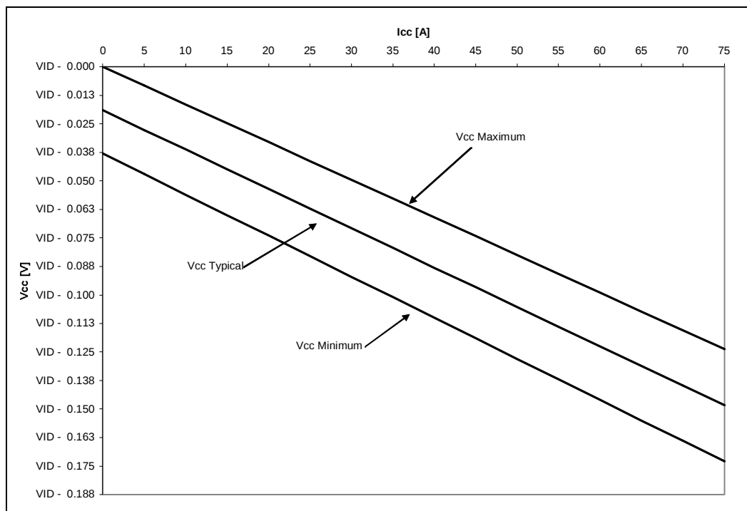
Figure 1. Processor V_{CC} Static and Transient Tolerance
