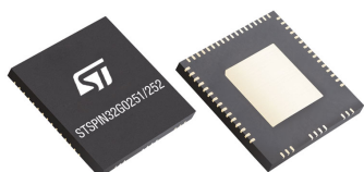
QFN 10x10 72L pitch 0.5
